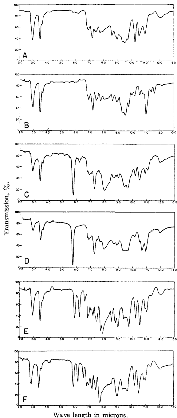
Fig. 1.—Infrared spectra in chloroform: A, zygadenine; B, pseudozygadenine; C, zygadenine triacetate; D, pseudozygadenine triacetate; E, veratrolyzgyadenine; F, vanillolyzgyadenine.
